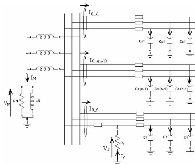
Fig. 1. A radial distribution network with an SLG fault.
