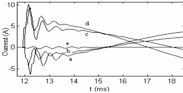
Fig. 8 Faulty (“c” and “d”) and sound current residuals in radial five feeders system of Fig. 5, with 30km overhead lines replacing cables on feeders “d” and “e”, an SLG fault on “d”. R_f=1k\Omega , \theta=90^\circ
