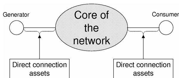
Figure 3 Distinction between connection lines and core of the network
