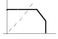
Fig. 2. Rate region: equal rates are not maxmin fair
