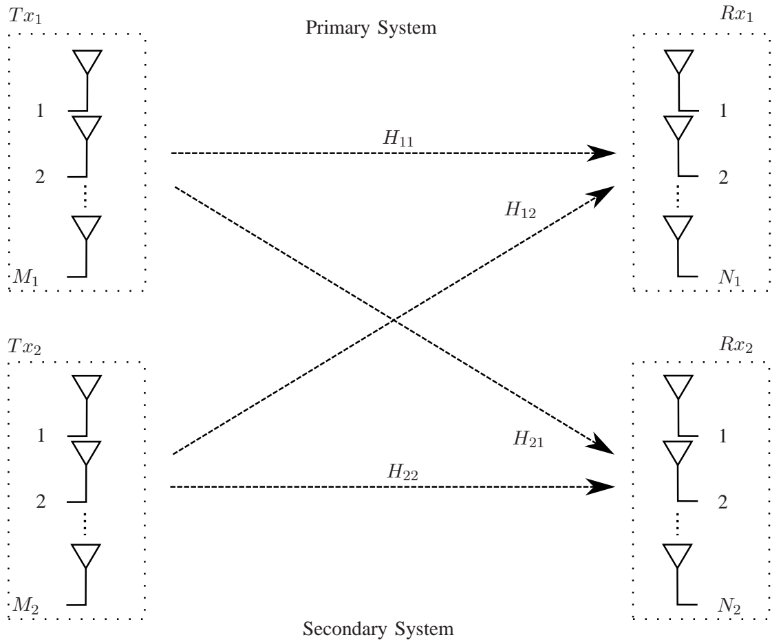
Figure 1. Two-user MIMO interference channel.
