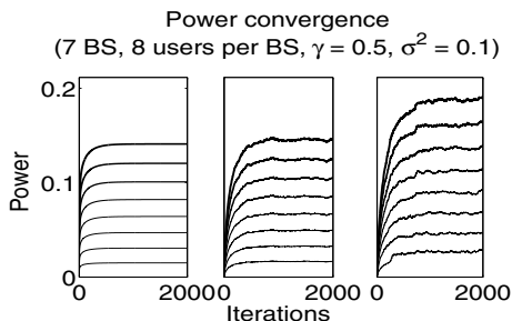
Fig. 3. Power convergence for Systems S1, S2 and S3 (H1 Network)
