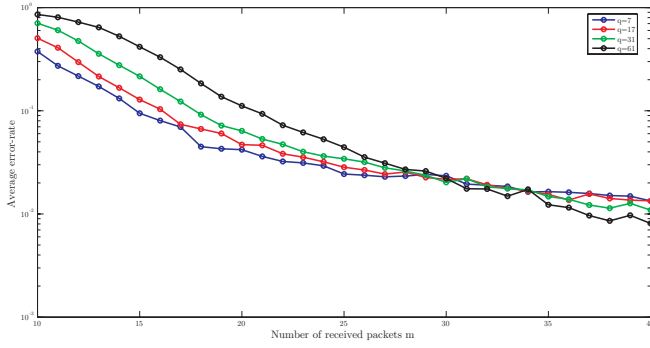
Fig. 3. Probability of reconstruction packets error as a function of the number m of received packets for various field size
