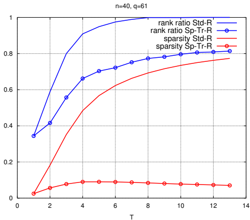
Fig. 2. Performance of the sparse-transfer routing algorithm.
