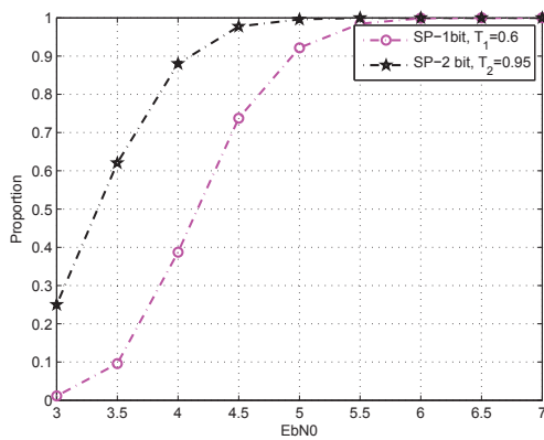
Fig. 5. Proportion of frames above threshold vs E_b/N_0
