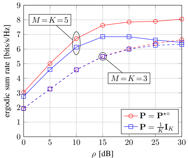
Fig. 8. RZF-CDU, R_{\text{sum}} vs. \rho with \alpha=1/\rho , \Theta_k = \mathbf{I}_M \forall k , P=1 and \tau_k^2 \in \mathcal{T}_1, \cup_{k=1}^3 \tau_k^2 = \mathcal{T}_1 ( M=5 ) and \tau_k^2 \in \mathcal{T}_2, \cup_{k=1}^3 \tau_k^2 = \mathcal{T}_2 ( M=3 ).
