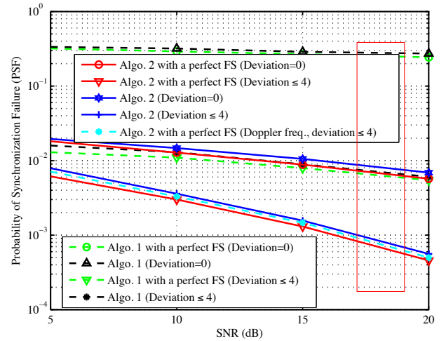
Figure 7. Probability of Synchronization Failure (the rectangular box presents the operating area of the 802.11a standard).
