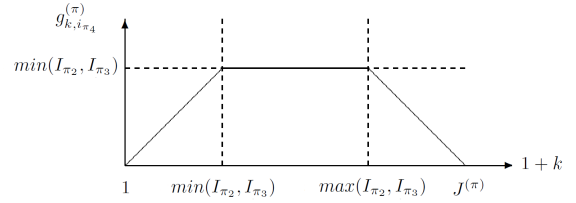
Figure 3. Number of occurrences g_{k, i_{\pi_4}}^{(\pi)} of the columns \mathbf{G}_{i_{\pi_4}}^{(\pi)}(:, k) for k \in \{1, \dots, J^{(\pi)}\} in the matrix [\mathcal{A}_{:, :, :, i_{\pi_4}}]_{\pi_1}
